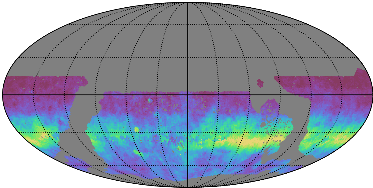
too_10_4v3.4_10yrs WFD r band: AngleRms rotSkyPos
