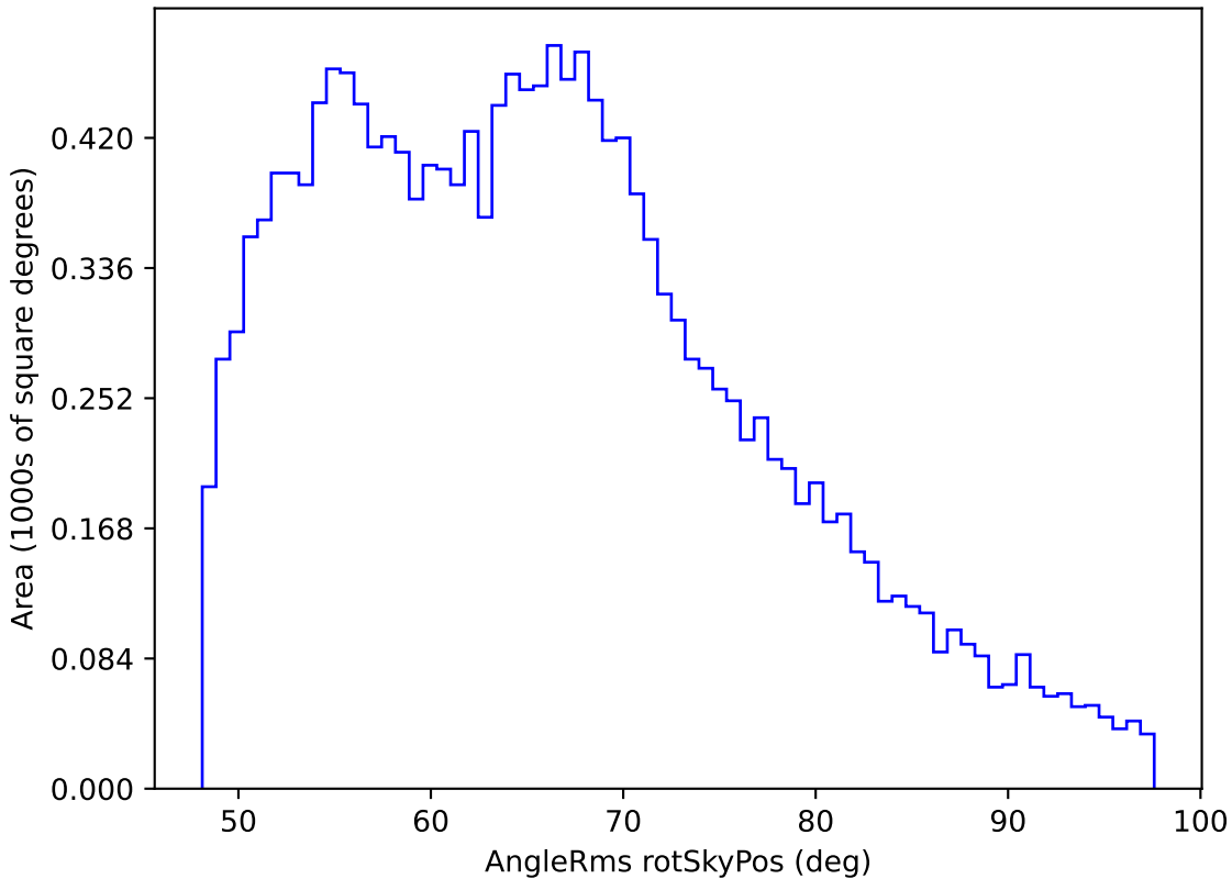
too_10_4v3.4_10yrs WFD r band: AngleRms rotSkyPos
