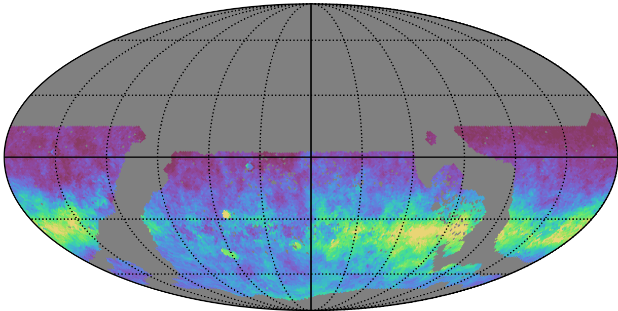
too_10_4v3.4_10yrs WFD i band: AngleRms rotSkyPos
