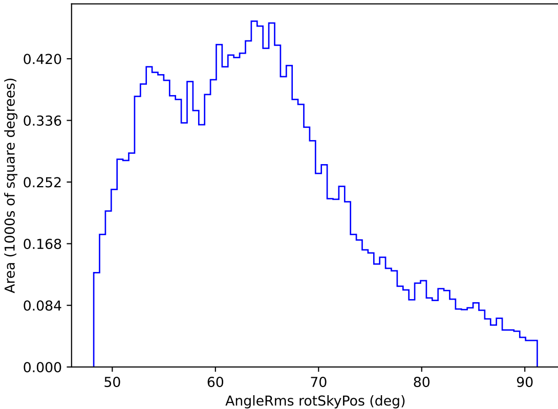
too_10_4v3.4_10yrs WFD i band: AngleRms rotSkyPos
