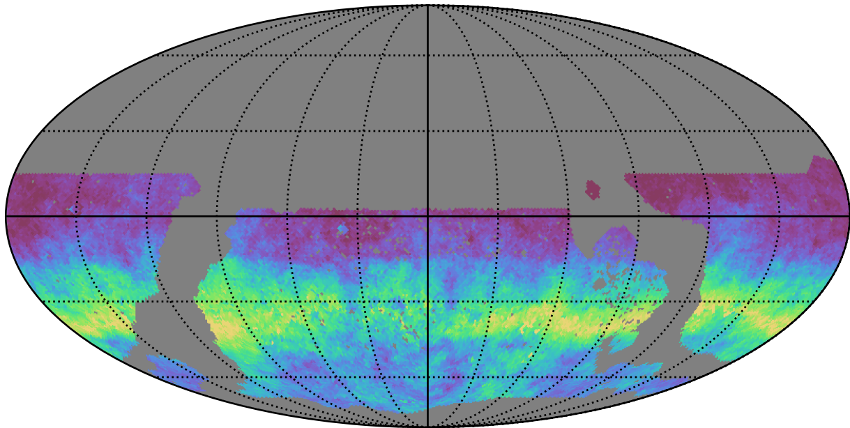
too_10_4v3.4_10yrs WFD g band: AngleRms rotSkyPos
