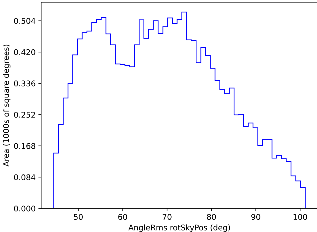
too_10_4v3.4_10yrs WFD g band: AngleRms rotSkyPos
