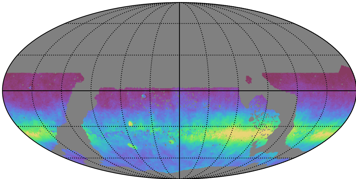
too_10_4v3.4_10yrs WFD all bands: AngleRms rotSkyPos
