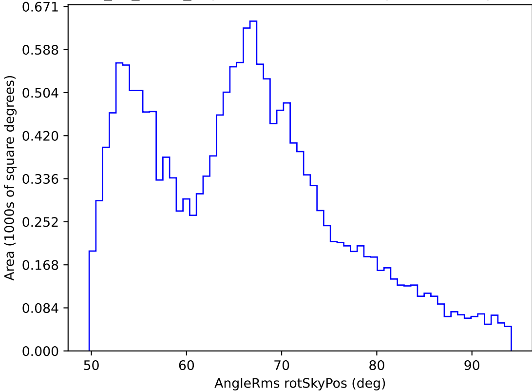
too_10_4v3.4_10yrs WFD all bands: AngleRms rotSkyPos
