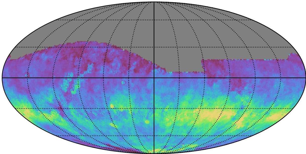
too_10_4v3.4_10yrs All sky z band: AngleRms rotSkyPos
