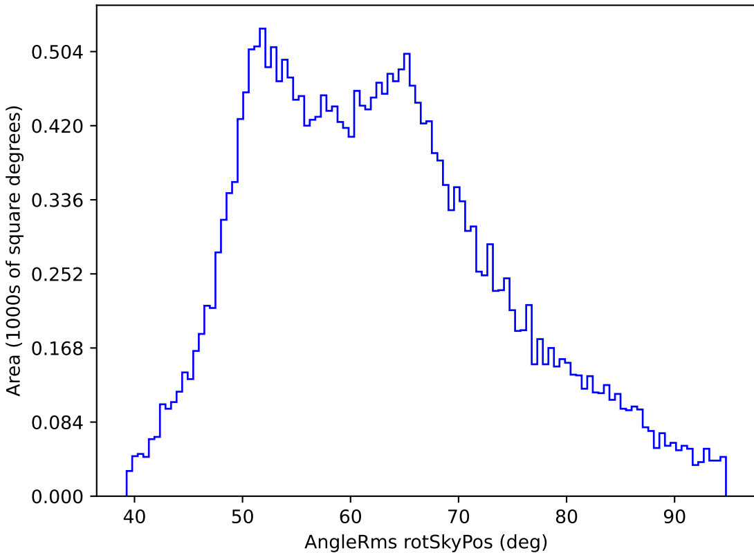
too_10_4v3.4_10yrs All sky z band: AngleRms rotSkyPos
