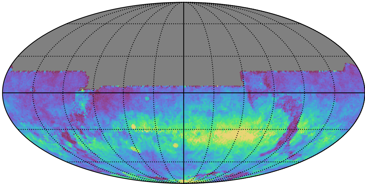
too_10_4v3.4_10yrs All sky y band: AngleRms rotSkyPos
