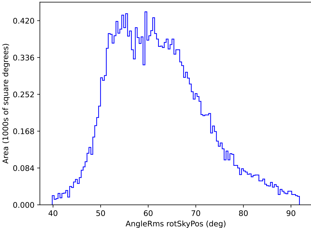
too_10_4v3.4_10yrs All sky y band: AngleRms rotSkyPos
