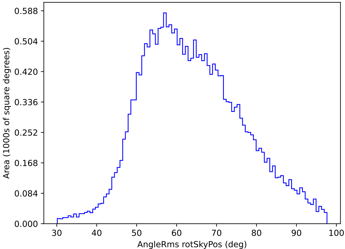
too_10_4v3.4_10yrs All sky u band: AngleRms rotSkyPos
