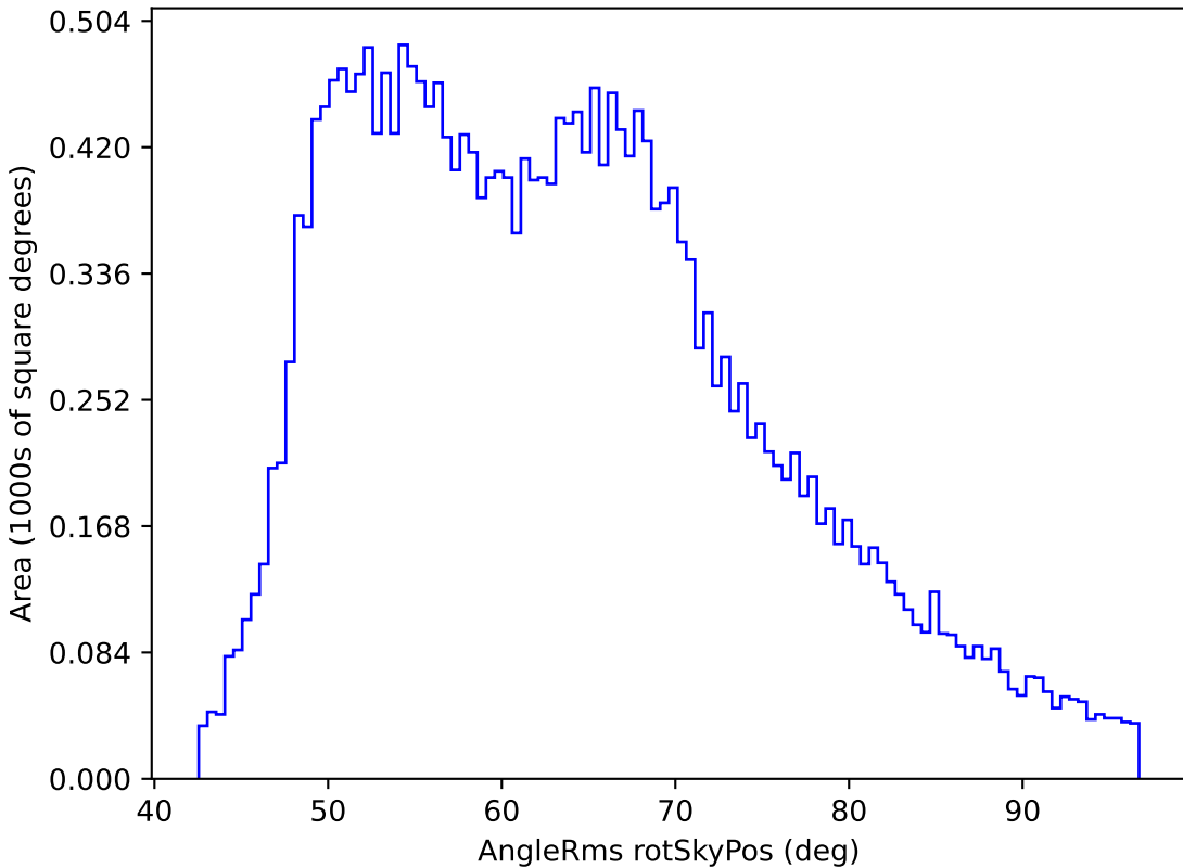
too_10_4v3.4_10yrs All sky r band: AngleRms rotSkyPos
