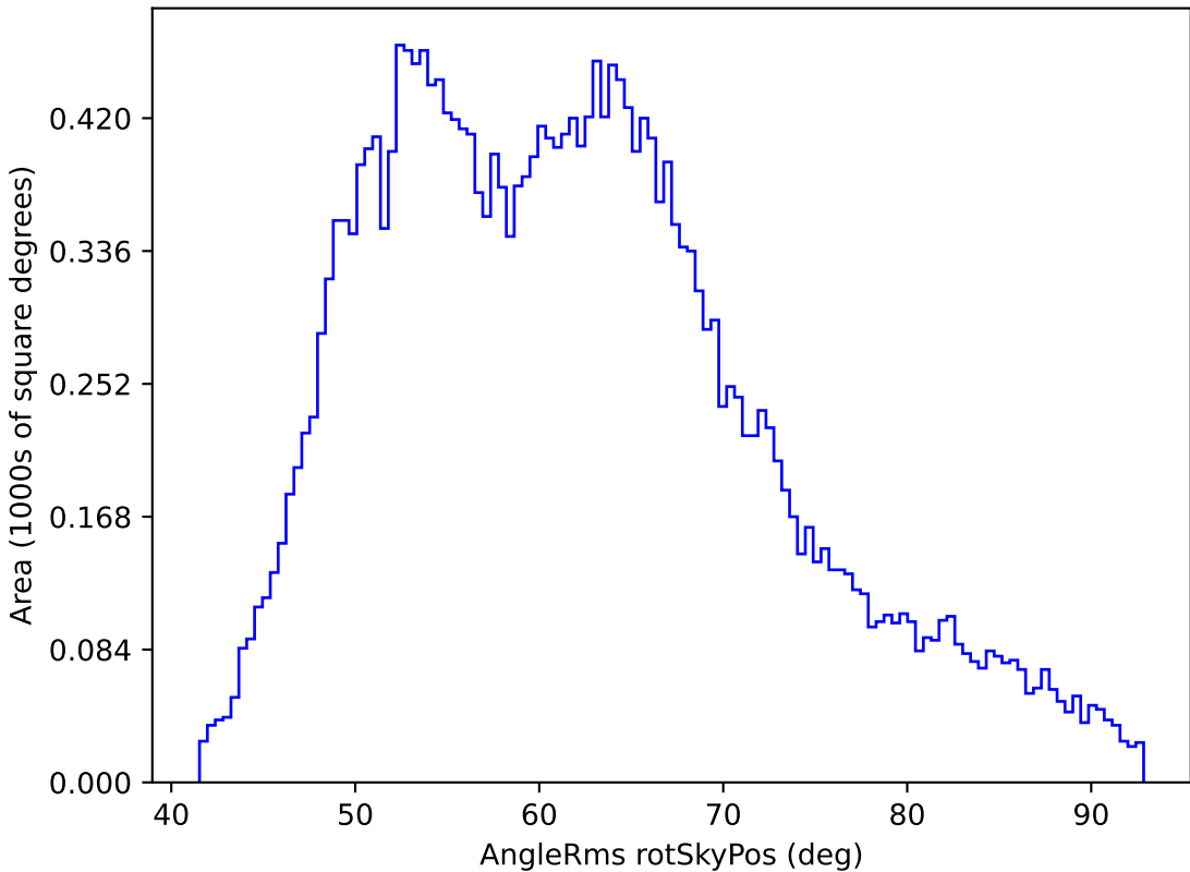
too_10_4v3.4_10yrs All sky i band: AngleRms rotSkyPos
