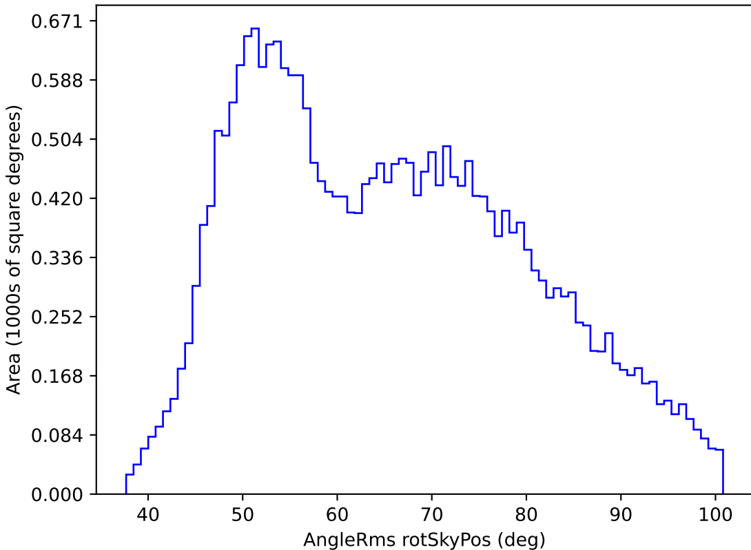
too_10_4v3.4_10yrs All sky g band: AngleRms rotSkyPos
