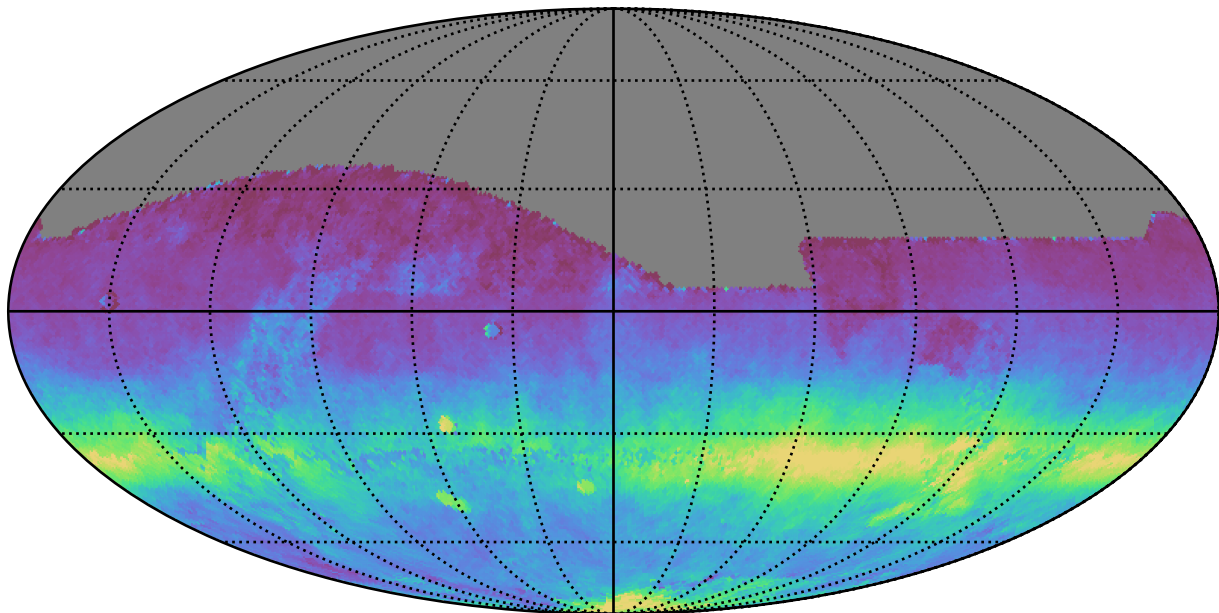
too_10_4v3.4_10yrs All sky all bands: AngleRms rotSkyPos
