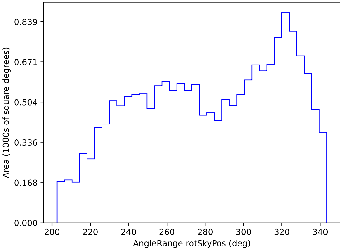
too_10_4v3.4_10yrs WFD z band: AngleRange rotSkyPos
