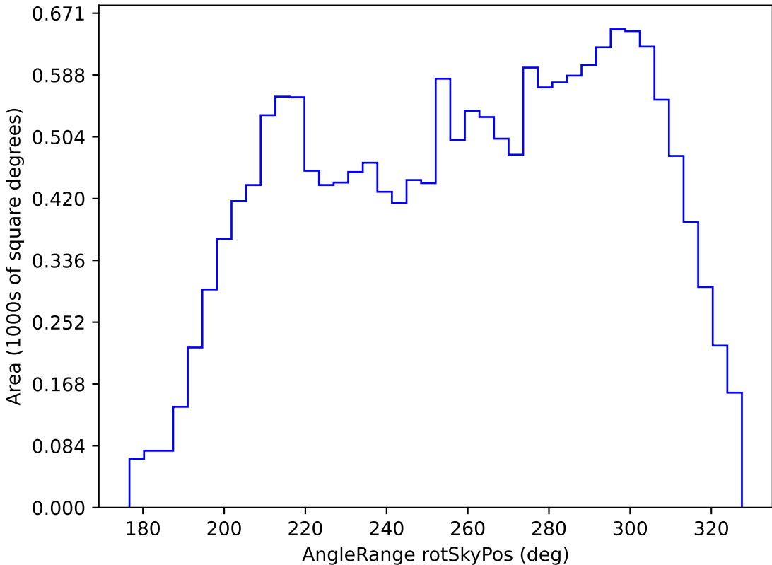
too_10_4v3.4_10yrs WFD u band: AngleRange rotSkyPos
