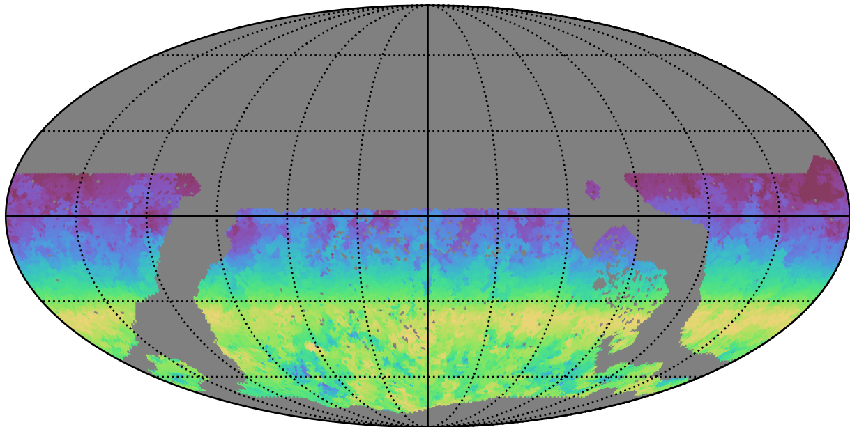
too_10_4v3.4_10yrs WFD r band: AngleRange rotSkyPos
