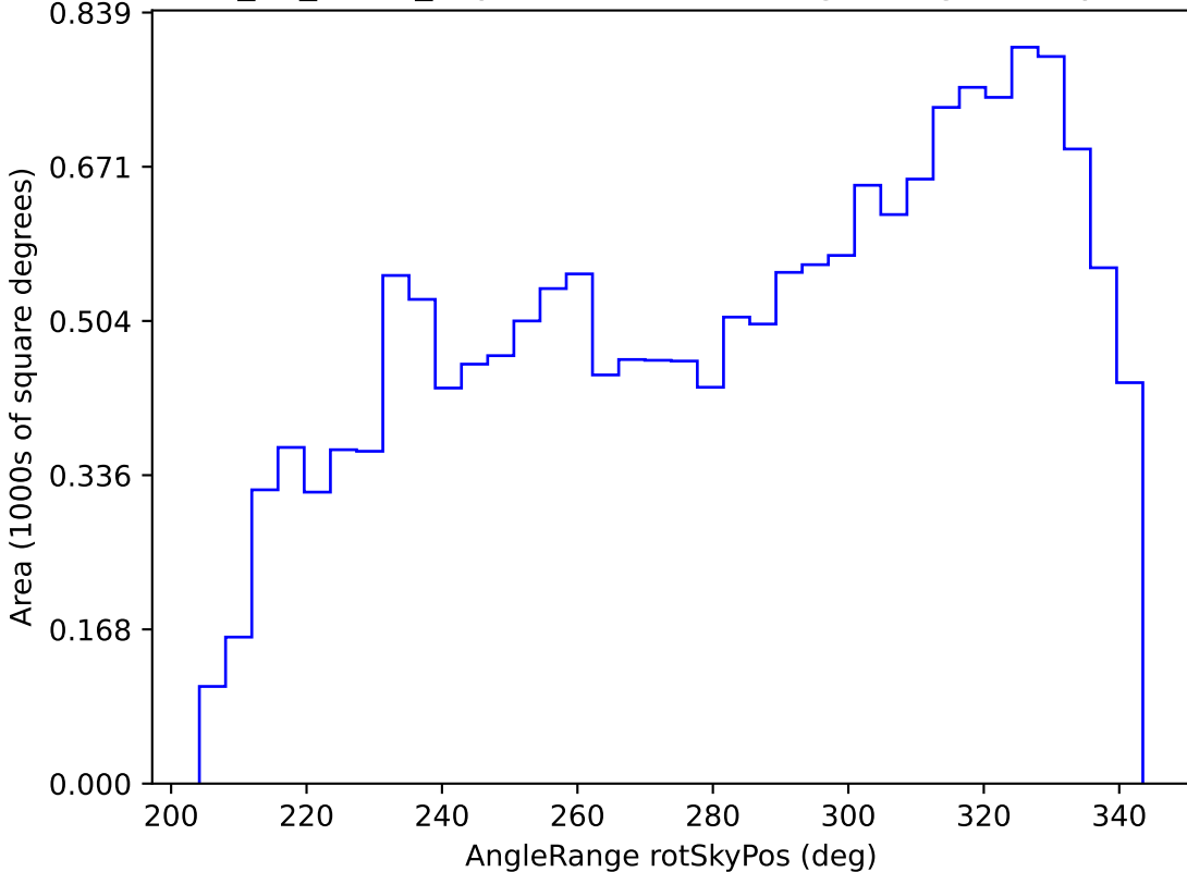
too_10_4v3.4_10yrs WFD r band: AngleRange rotSkyPos
