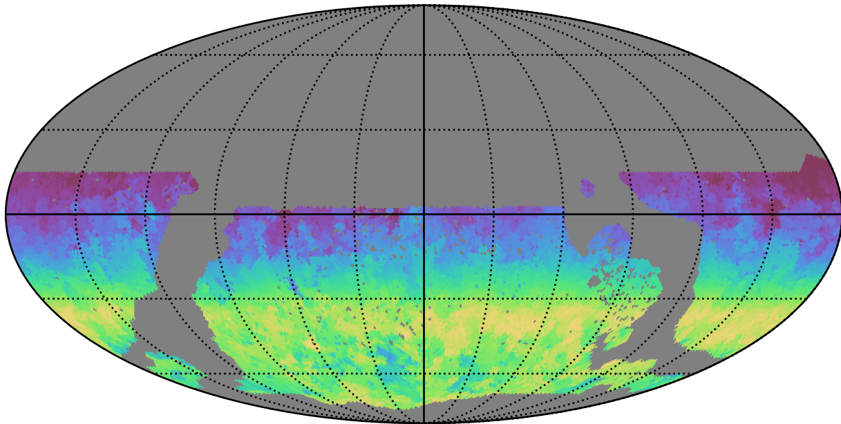
too_10_4v3.4_10yrs WFD i band: AngleRange rotSkyPos
