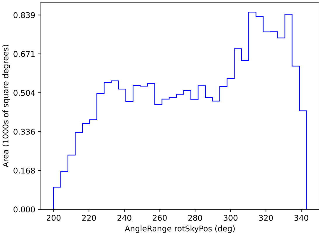
too_10_4v3.4_10yrs WFD i band: AngleRange rotSkyPos
