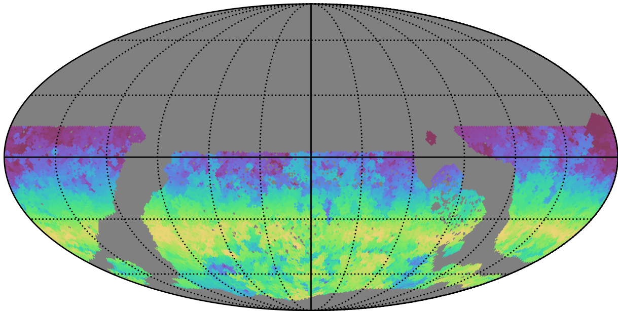
too_10_4v3.4_10yrs WFD g band: AngleRange rotSkyPos
