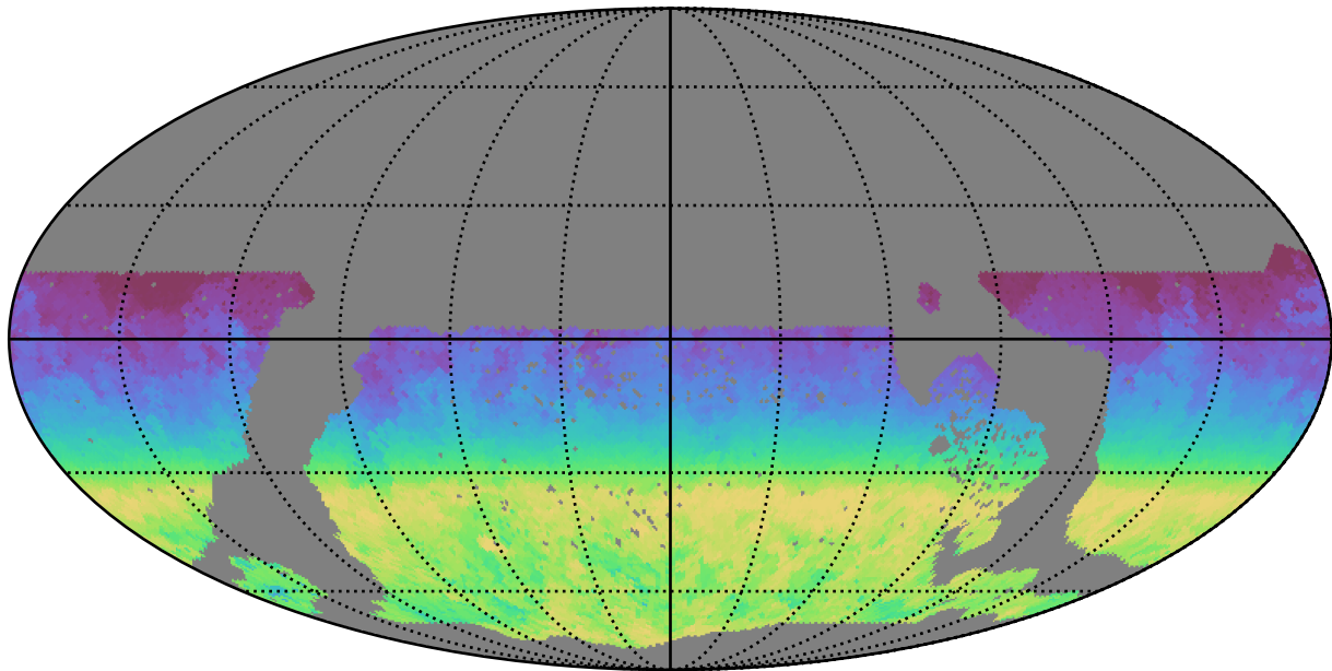
too_10_4v3.4_10yrs WFD all bands: AngleRange rotSkyPos
