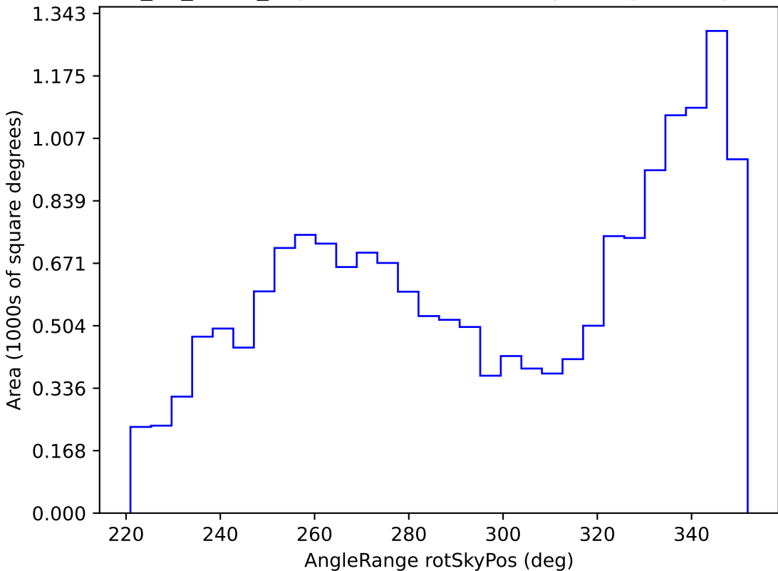
too_10_4v3.4_10yrs WFD all bands: AngleRange rotSkyPos
