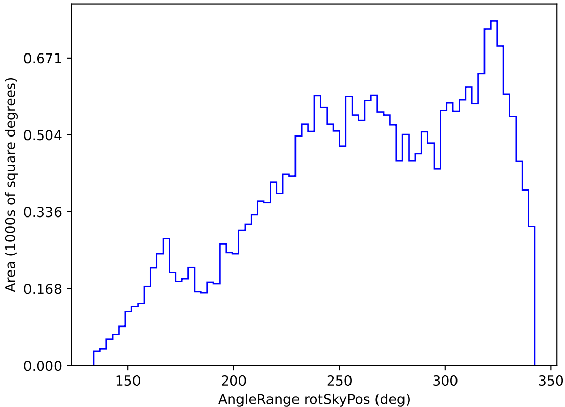
too_10_4v3.4_10yrs All sky z band: AngleRange rotSkyPos
