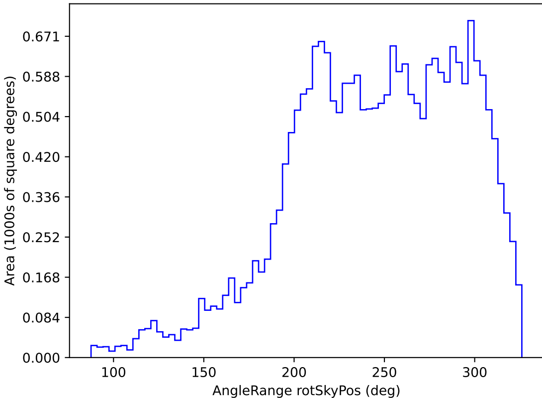
too_10_4v3.4_10yrs All sky u band: AngleRange rotSkyPos
