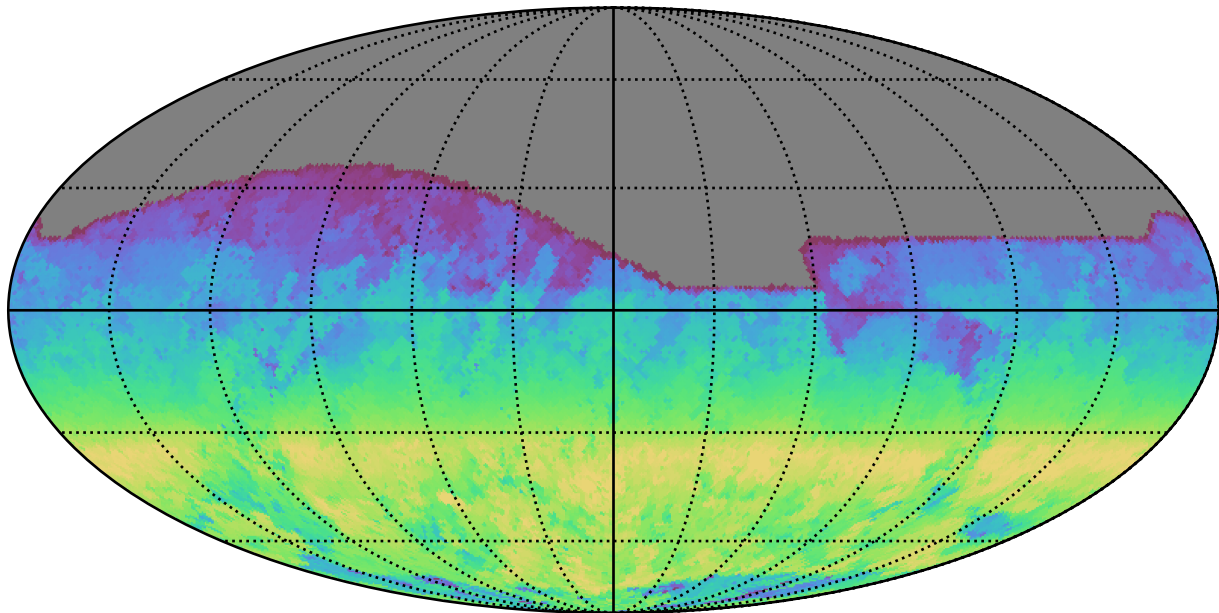
too_10_4v3.4_10yrs All sky r band: AngleRange rotSkyPos
