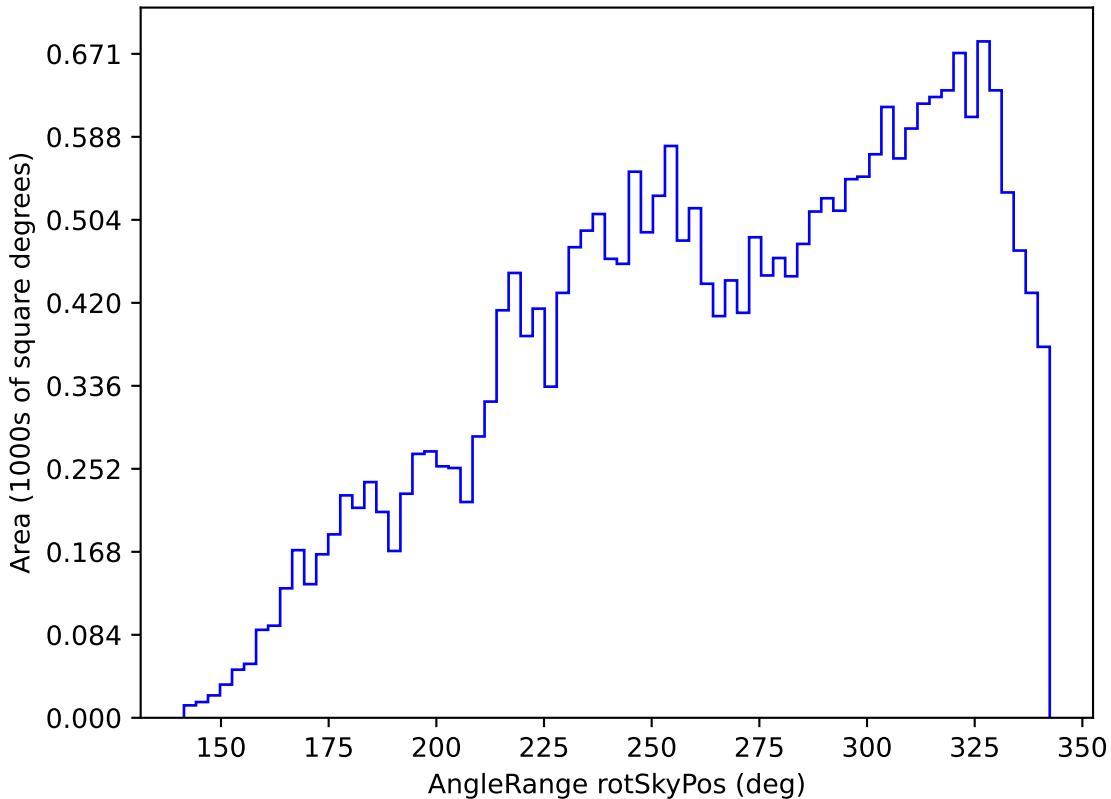
too_10_4v3.4_10yrs All sky r band: AngleRange rotSkyPos
