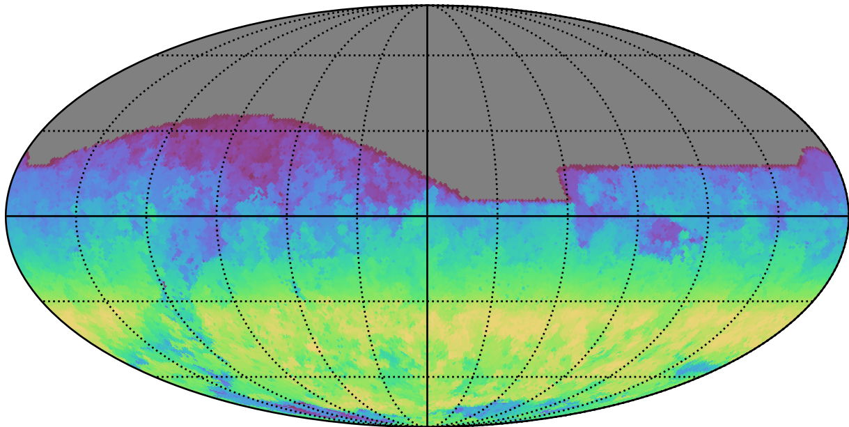
too_10_4v3.4_10yrs All sky i band: AngleRange rotSkyPos
