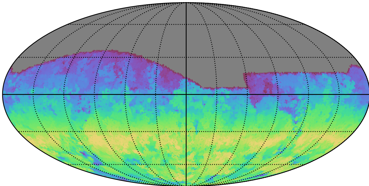
too_10_4v3.4_10yrs All sky g band: AngleRange rotSkyPos
