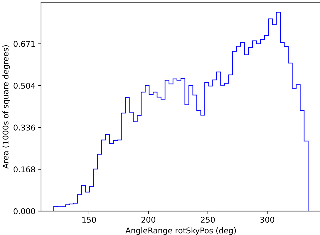
too_10_4v3.4_10yrs All sky g band: AngleRange rotSkyPos
