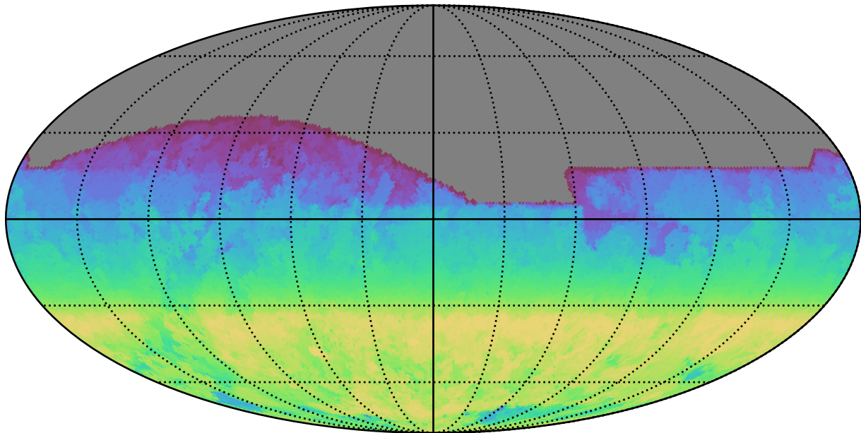
too_10_4v3.4_10yrs All sky all bands: AngleRange rotSkyPos
