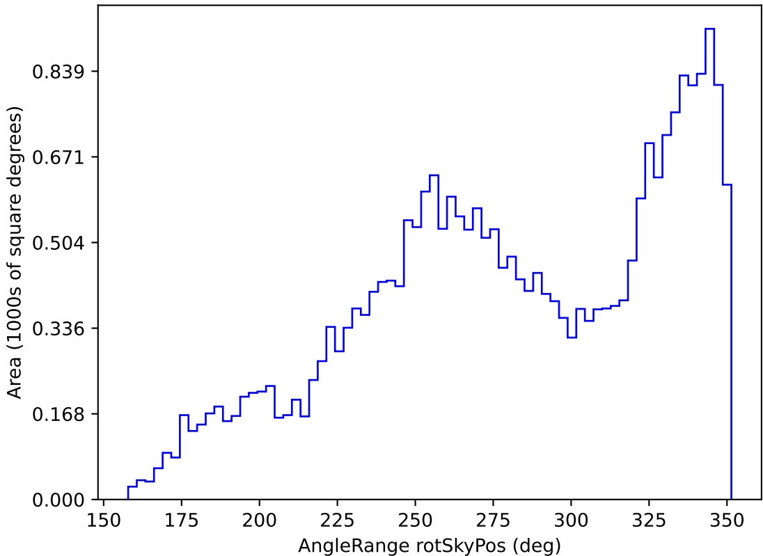
too_10_4v3.4_10yrs All sky all bands: AngleRange rotSkyPos
