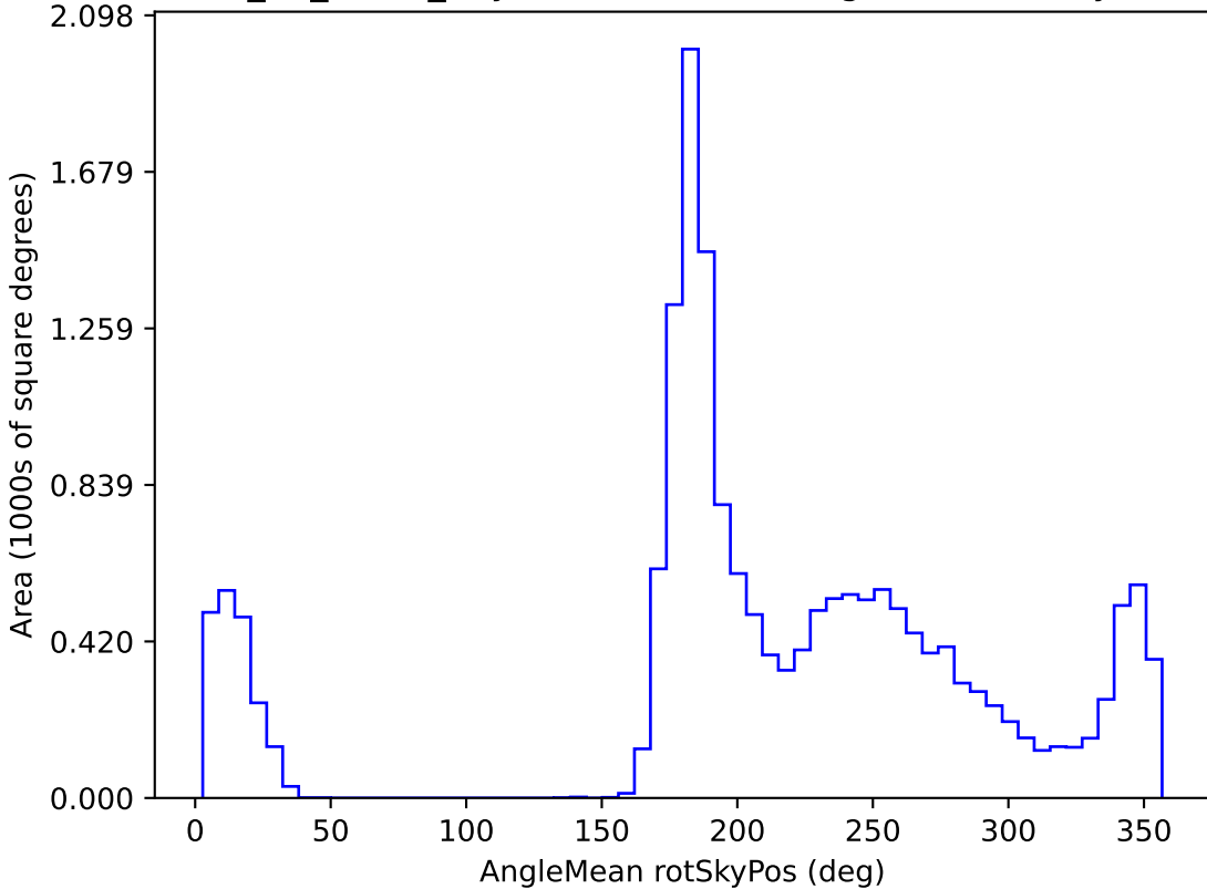
too_10_4v3.4_10yrs WFD z band: AngleMean rotSkyPos
