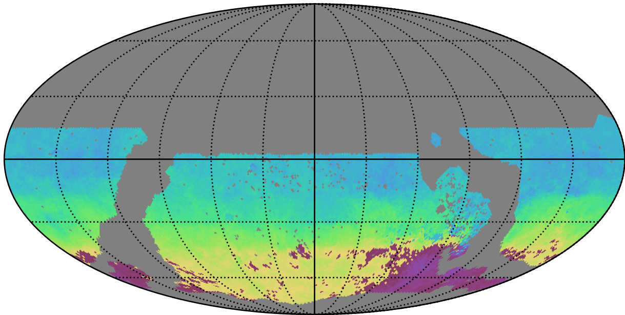
too_10_4v3.4_10yrs WFD u band: AngleMean rotSkyPos
