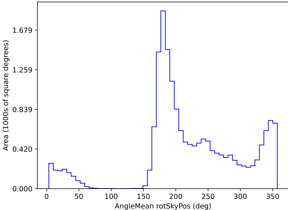
too_10_4v3.4_10yrs WFD u band: AngleMean rotSkyPos
