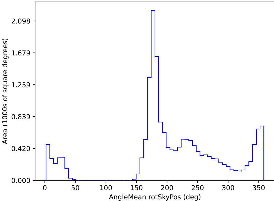
too_10_4v3.4_10yrs WFD r band: AngleMean rotSkyPos
