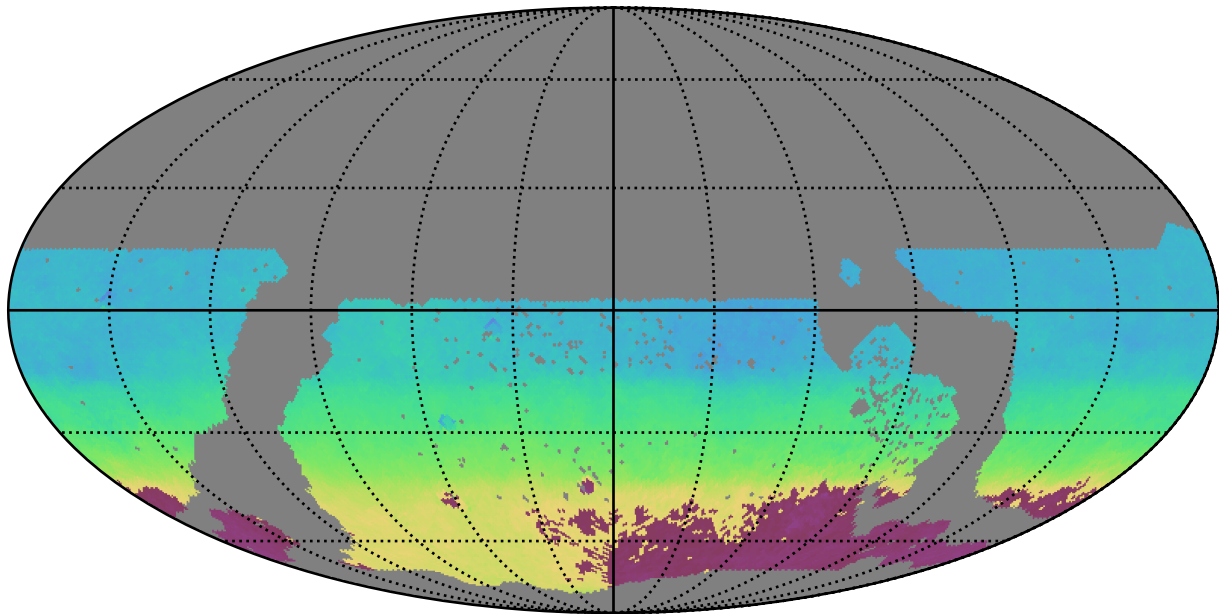
too_10_4v3.4_10yrs WFD i band: AngleMean rotSkyPos
