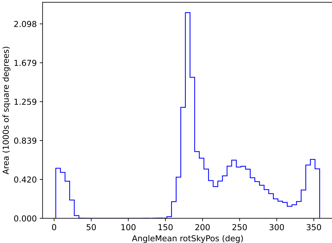
too_10_4v3.4_10yrs WFD i band: AngleMean rotSkyPos
