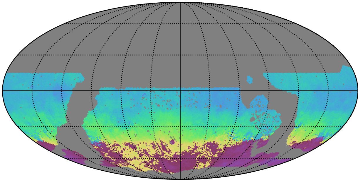
too_10_4v3.4_10yrs WFD g band: AngleMean rotSkyPos
