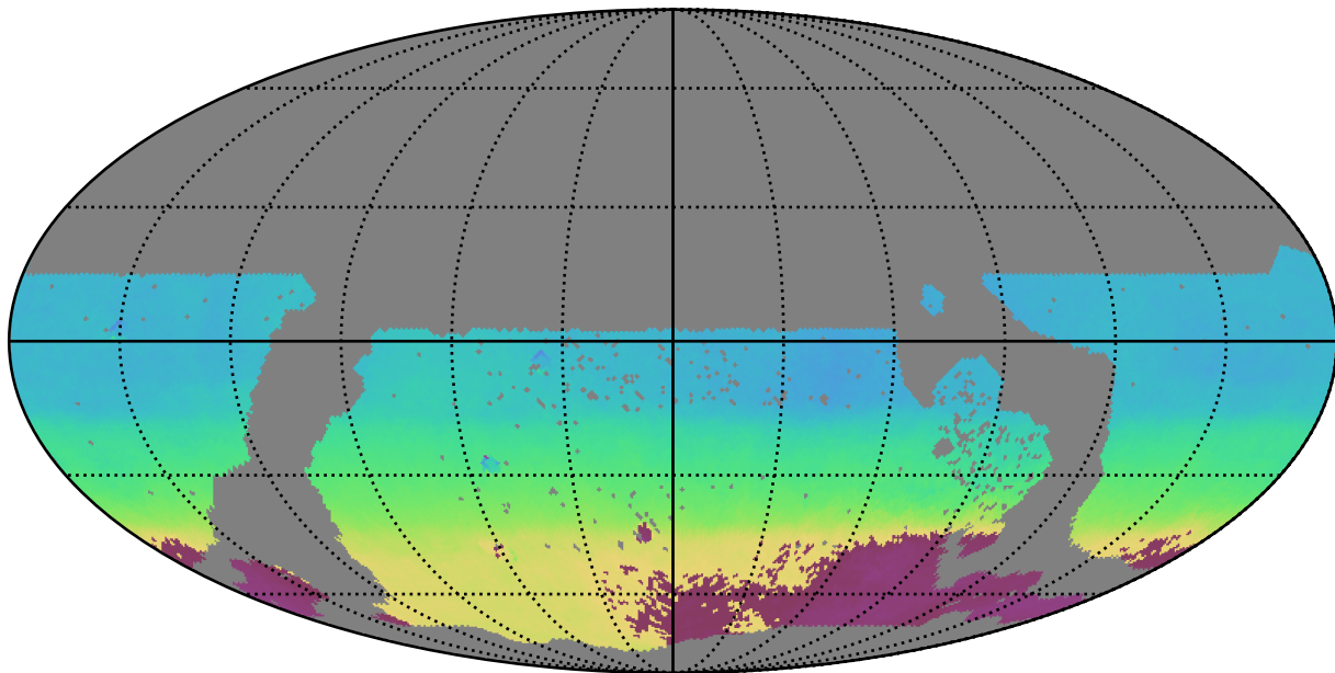
too_10_4v3.4_10yrs WFD all bands: AngleMean rotSkyPos
