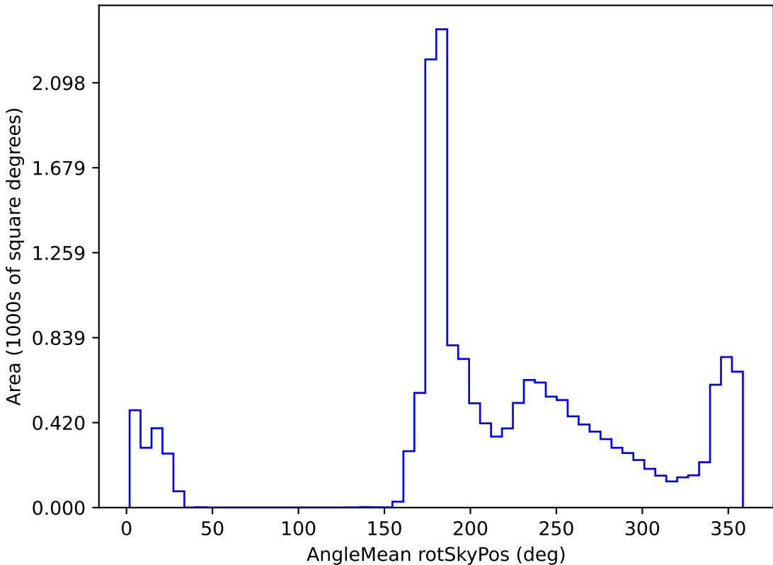
too_10_4v3.4_10yrs WFD all bands: AngleMean rotSkyPos
