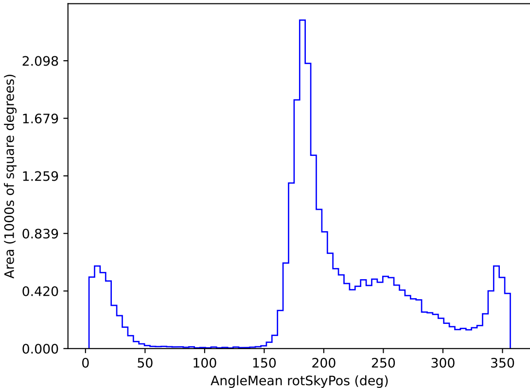
too_10_4v3.4_10yrs All sky z band: AngleMean rotSkyPos
