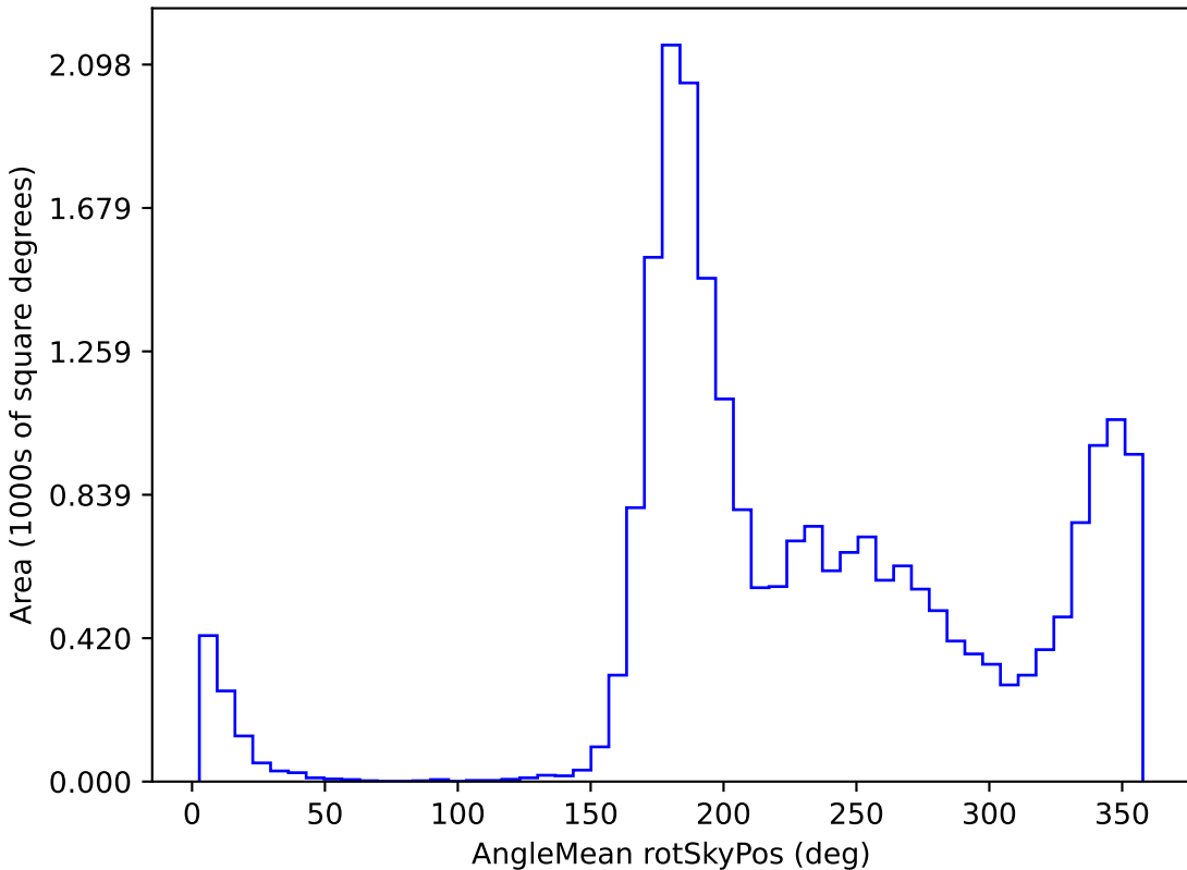
too_10_4v3.4_10yrs All sky y band: AngleMean rotSkyPos
