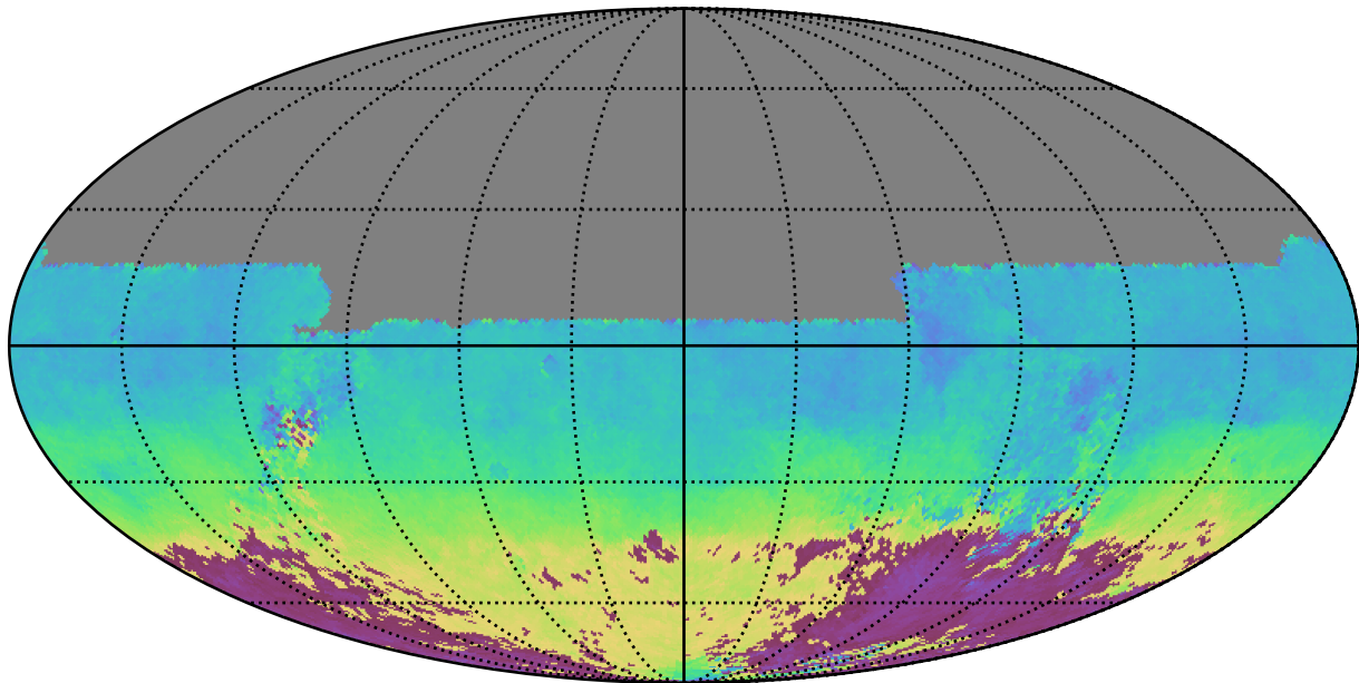
too_10_4v3.4_10yrs All sky u band: AngleMean rotSkyPos
