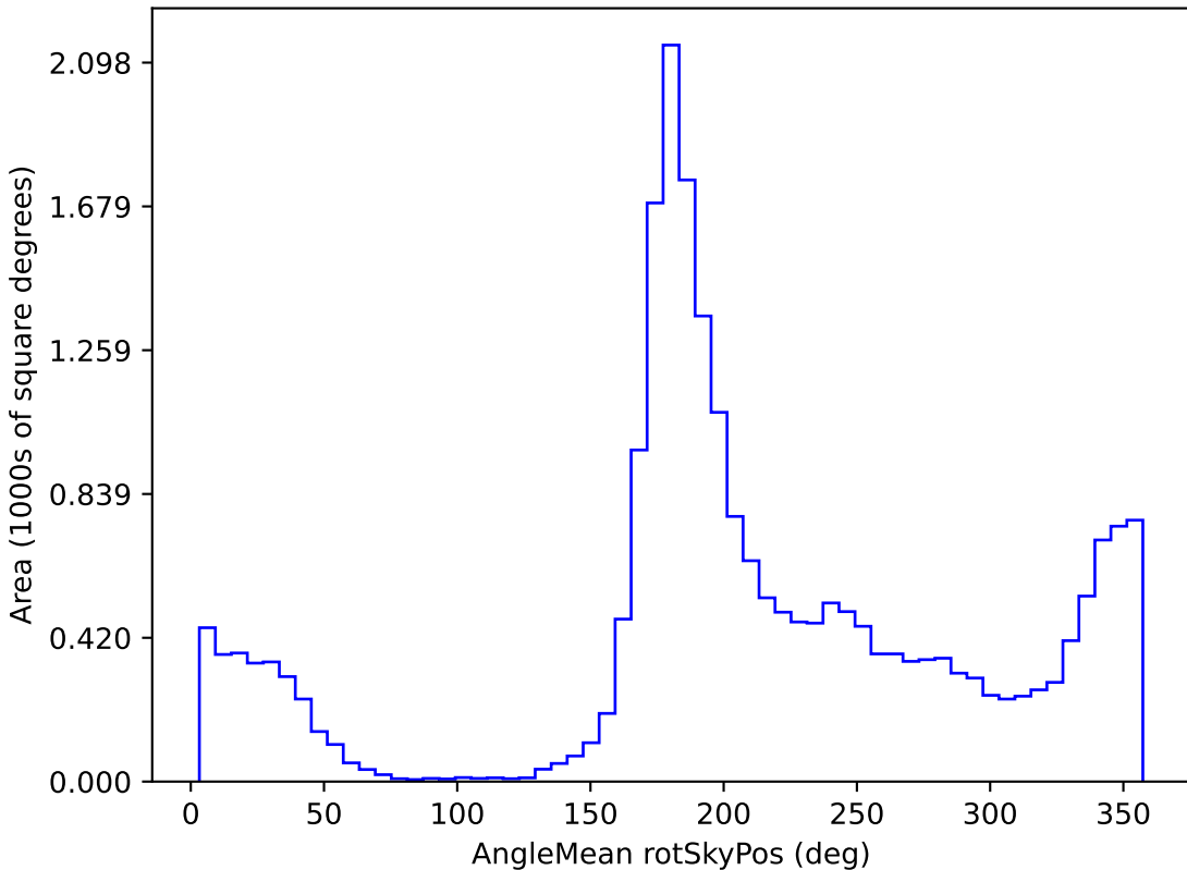
too_10_4v3.4_10yrs All sky u band: AngleMean rotSkyPos
