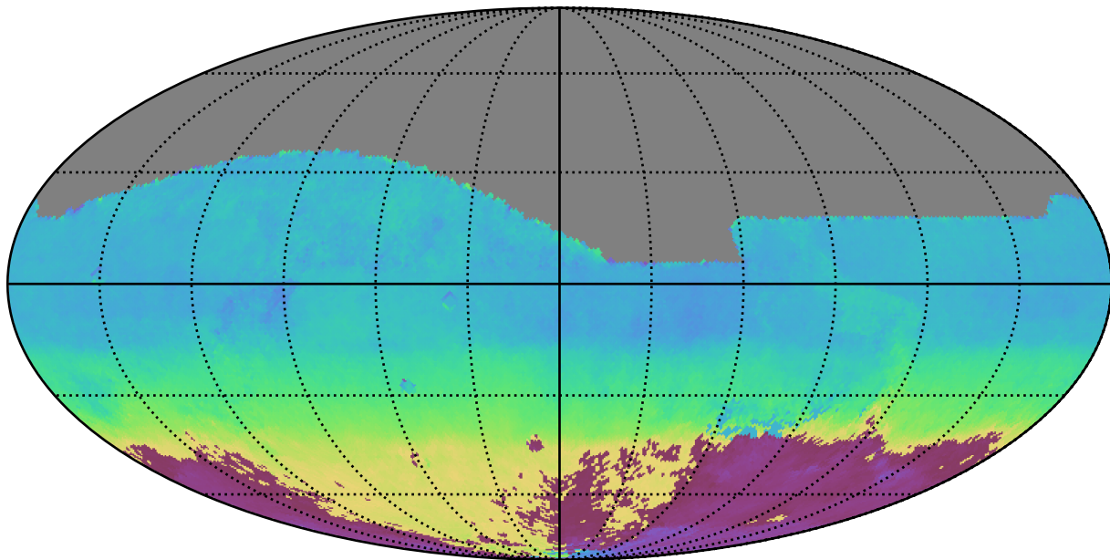
too_10_4v3.4_10yrs All sky r band: AngleMean rotSkyPos
