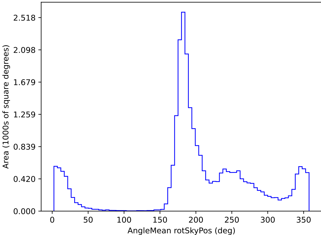
too_10_4v3.4_10yrs All sky i band: AngleMean rotSkyPos
